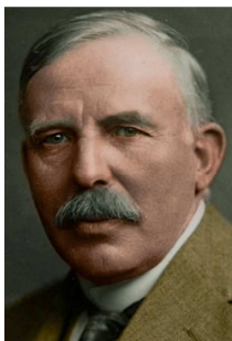
Ernest Rutheford 1871-1937
